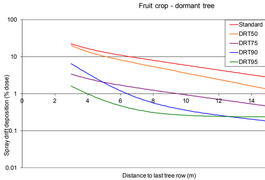
Figure 11 Spray drift deposition curves for the reference and typical 50%, 75%, 90% and 95% drift reduction classes application techniques in orchard spraying (dormant situation).
