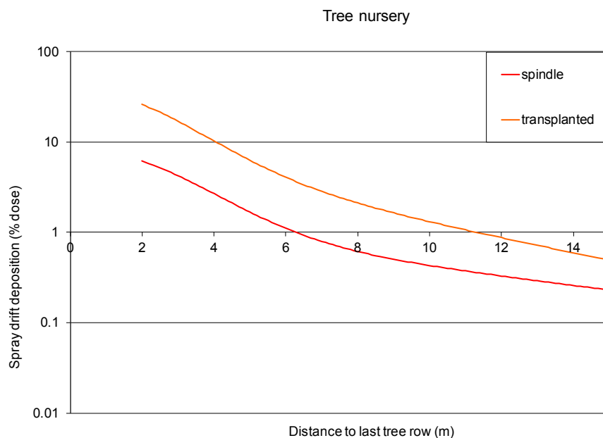
Figure 12 Standard spray drift deposition curves for the standard axial-fan spray techniques used in spindle and transplanted nursery trees.
